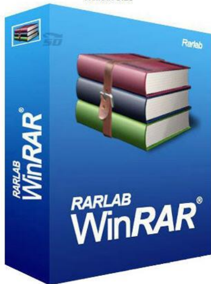
WinRAR 5.21
